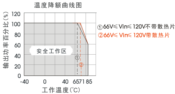
URB1D03LD-20W(H)R3(A2S/A4S)工作温度曲线
