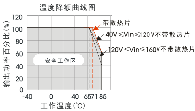
URB1D03LD-20W(H)R3(A2S/A4S)工作温度曲线
